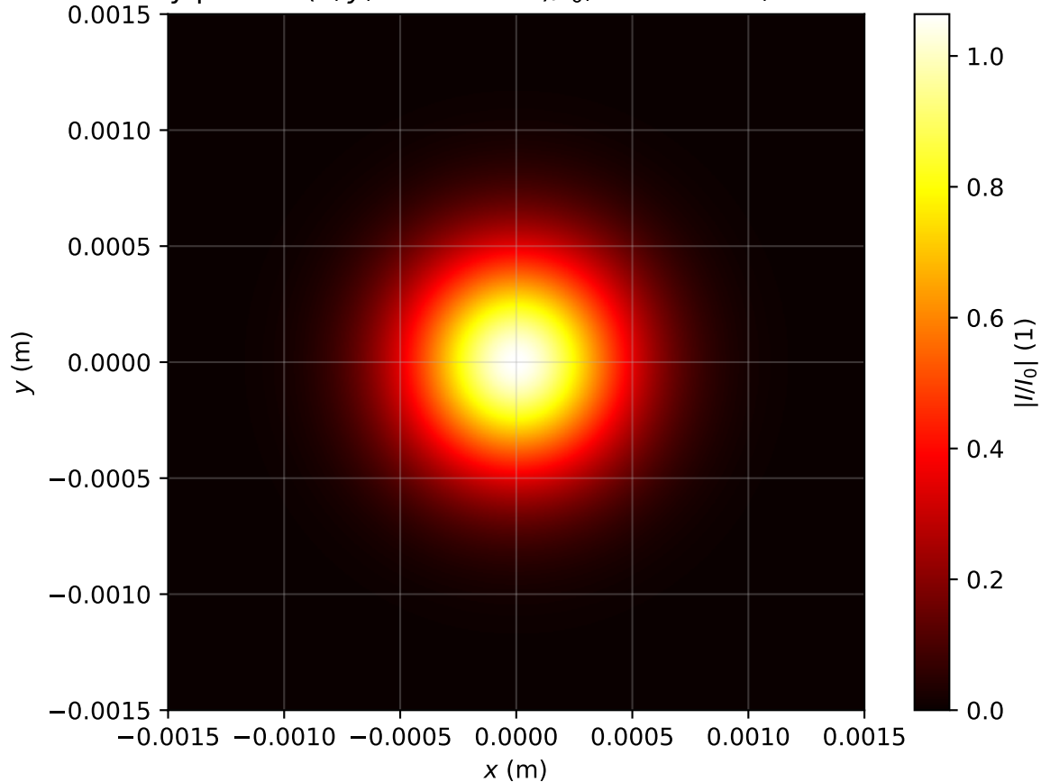
Intensity profile I(x, y, z = 0.318m)/I_0 , P_{in}=0.9P_{cr} , artificial time
